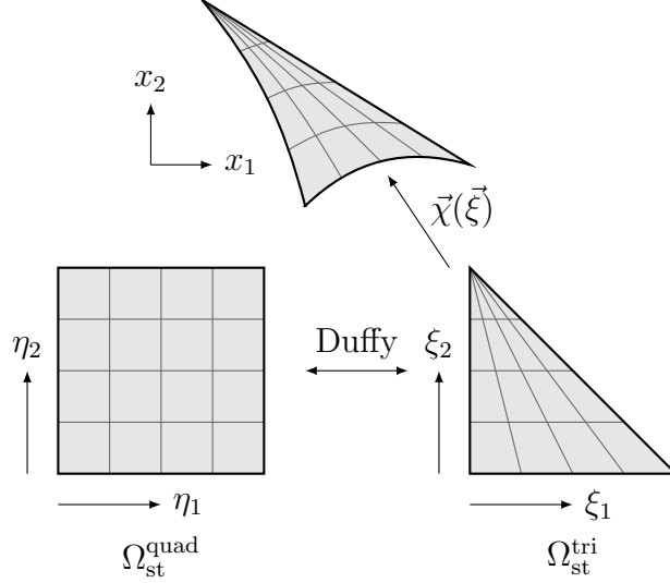
Figure 1: Duffy transformation from the standard quadrilateral element \Omega_{\text{st}}^{\text{quad}} with collapsed coordinates (\eta_1, \eta_2) to triangular element \Omega_{\text{st}}^{\text{tri}} with coordinates (\xi_1, \xi_2) . We also show how \Omega_{\text{st}}^{\text{tri}} is taken to a general curvilinear element through the isoparametric mapping \vec{\chi} . Interior lines demonstrate how quadrature points, taken to be equally spaced in this example, are transformed under each mapping.
