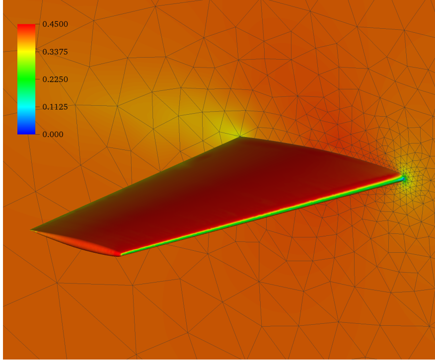
Figure 9: Distribution of the Mach number 0 < M \leq 0.45 across the surface of the ONERA M6 wing as the flow evolves to a steady state.
