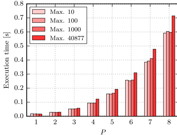
Figure 6: Effect of amalgamation sizes on the observed evaluation time for the inner product operator on tetrahedral elements.
