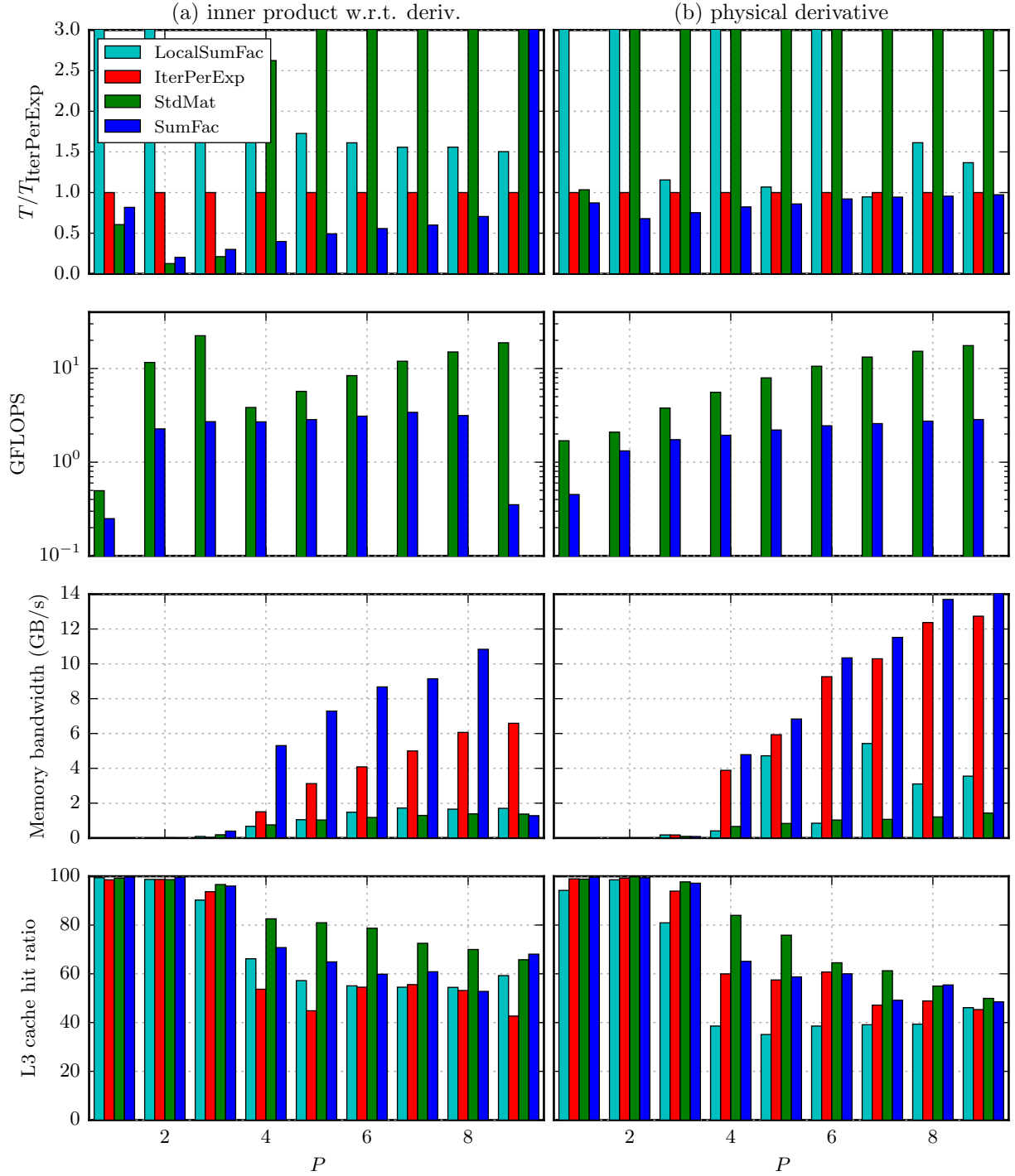
Figure 8: Measurements of runtime, GFLOPS, memory bandwidth and L3 cache hit ratios for prismatic elements under OpenBLAS on an Intel Core i7-5930K.
