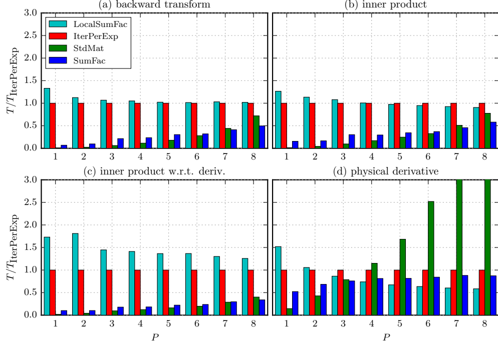
Figure 7: Performance characteristics for the four key operators with prismatic elements under OpenBLAS.
