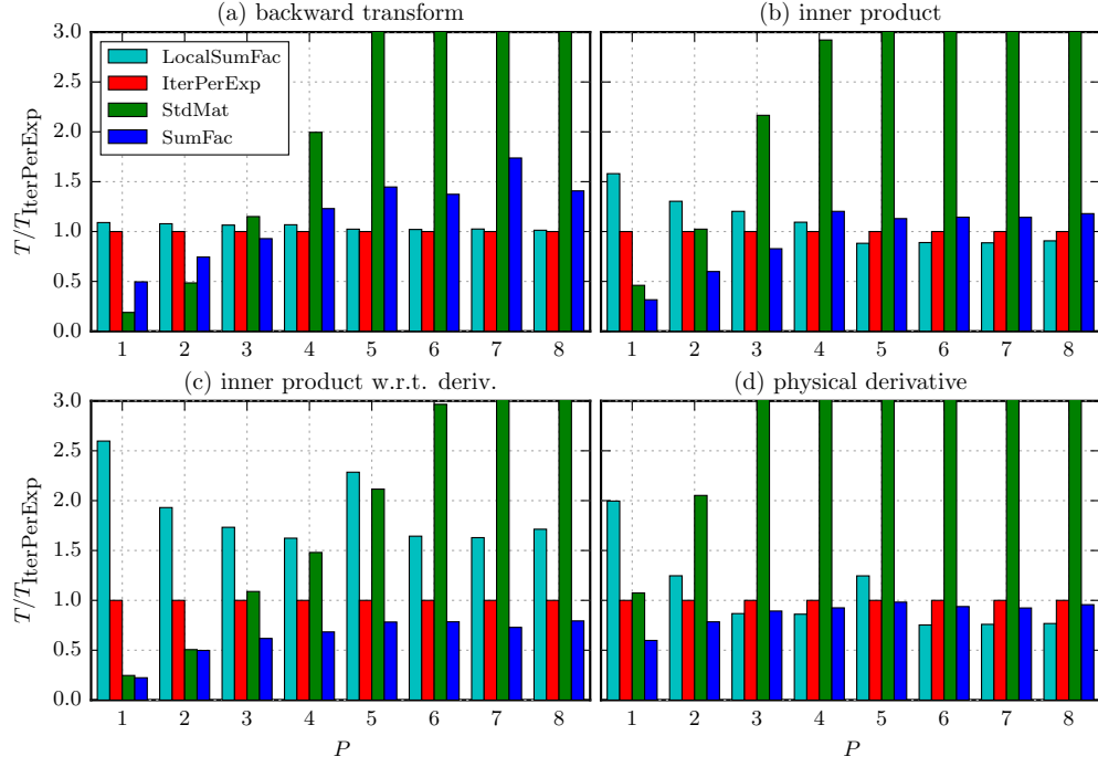
Figure 4: Initial performance characteristics for the four key operators with prismatic elements using the reference BLAS implementation from NETLIB.
