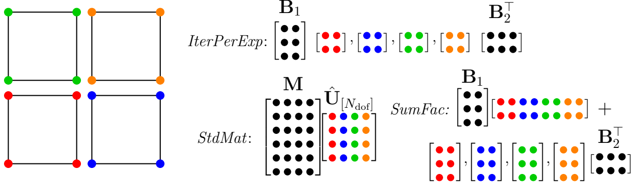
Figure 2: Diagrammatic representation of each amalgamation scheme. Four quadrilateral elements with P_1 = P_2 = 1 and Q_1 = Q_2 = 3 are considered for the backward transform operator.
