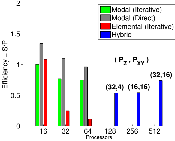
Figure 9: Turbulent pipe flow parallel simulation - efficiency of parallelisation approaches on a cluster of 8-core nodes. The histograms show the efficiency E of different parallel simulations defined as E = S/P where S is the speed-up and P is the total number of processors used for the simulation. The speed-up is based on the 16-core (2 nodes) run using the Modal (iterative) approach.
