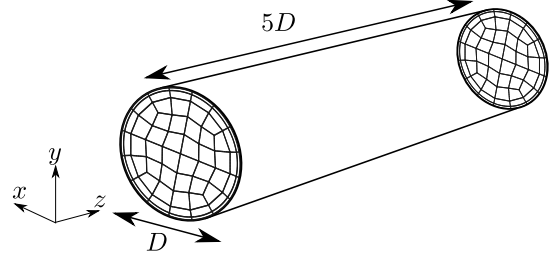
Figure 5: Diagram illustrating the pipe geometry and its discretisation. Spectral/hp elements are used in the cross-plane with a Fourier expansion used in the streamwise direction.
