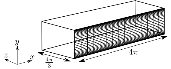
Figure 6: Diagram illustrating the channel geometry and its discretisation. A Fourier expansion is used in the spanwise direction.
